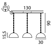
2199-10-10-K-130-3 Black Fixt. Antique Brass Shade, Chain Susp. 3x E27 max 18W Bulb excl.
