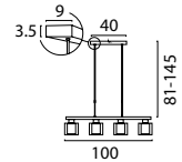
2890-05-05-100-4-14 Black Fixt. Black Cover, Telescopic Susp. 4x E27 max 18W Bulb excl.
