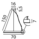
2795-05-70-DW-TR Black Fixt. Black Ring, Steel Wire, 56W 6270Lm 2700-2200K, Triac-Dim. On request:
