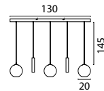
2341-05-05-1305RB220 Black, PVC cable, 3x E27 + 2x GU10 max 18W Bulb excl.
